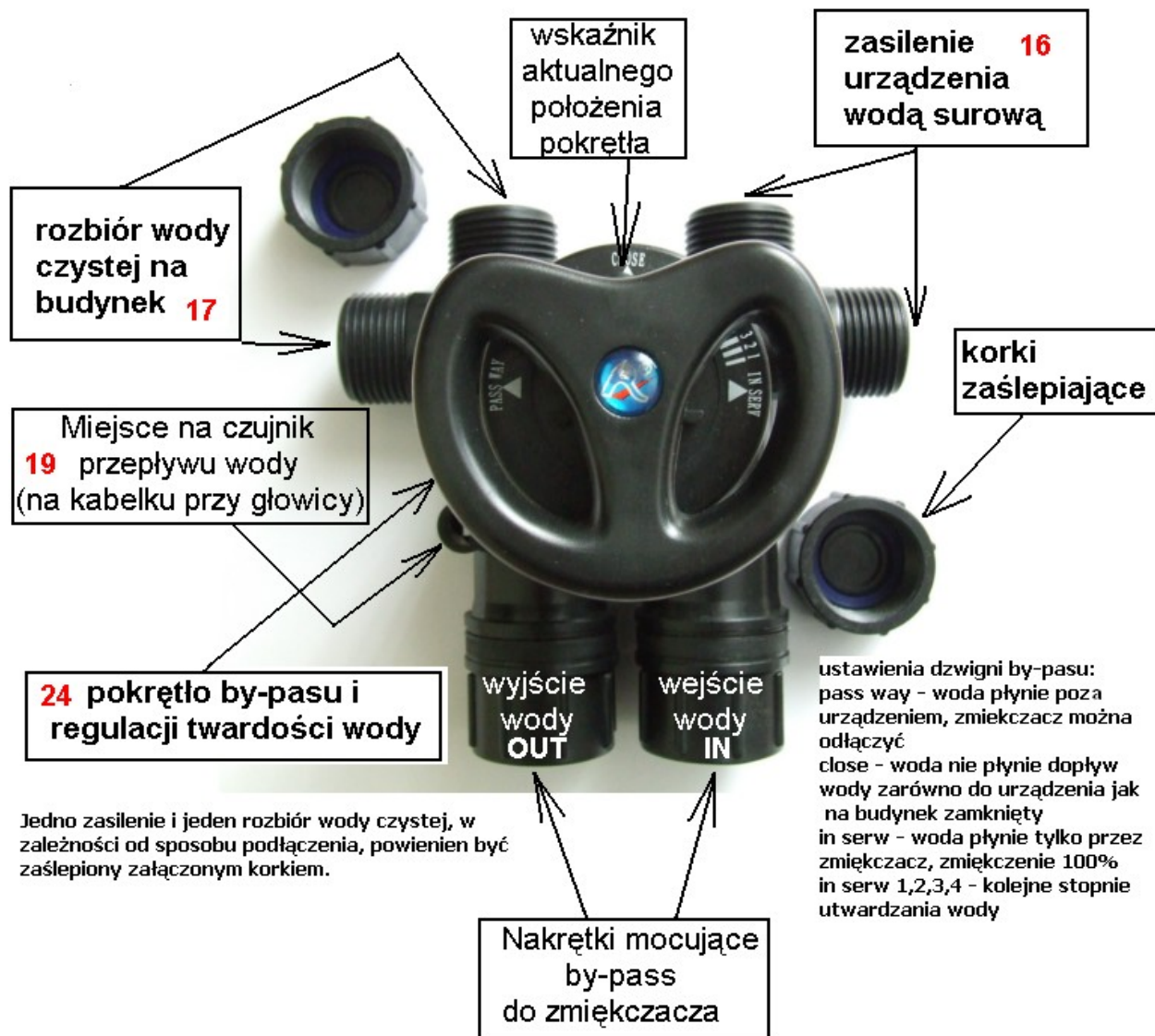
Rys. B. By-pass do sterownika RX68A-3+B
